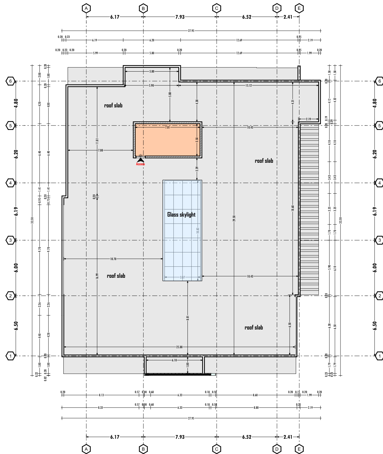
ROOF PLAN LAYOUT
