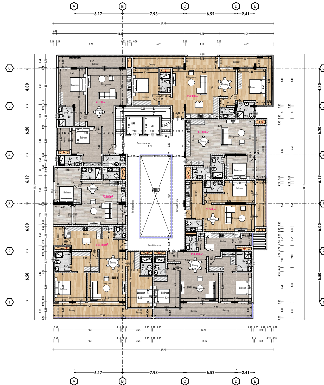
TYPICAL SECOND TO THIRD FLOOR PLAN
