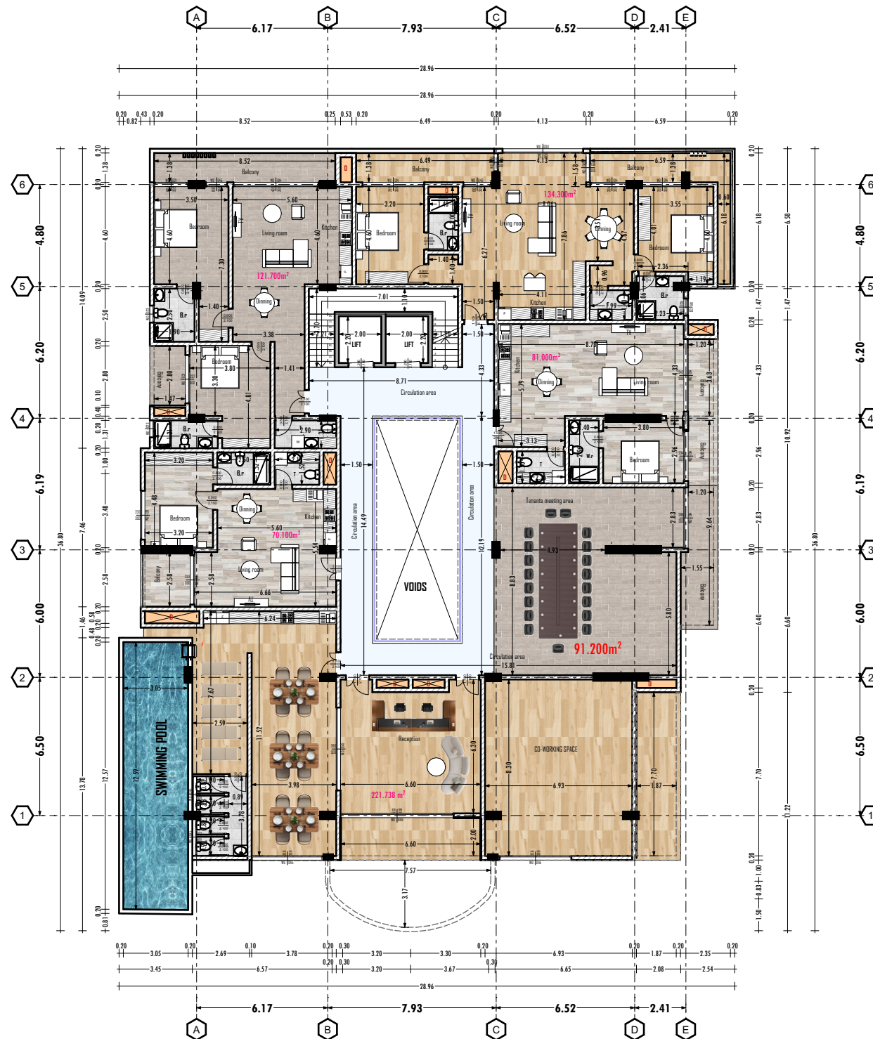
GROUND FLOOR PLAN LAYOUT
