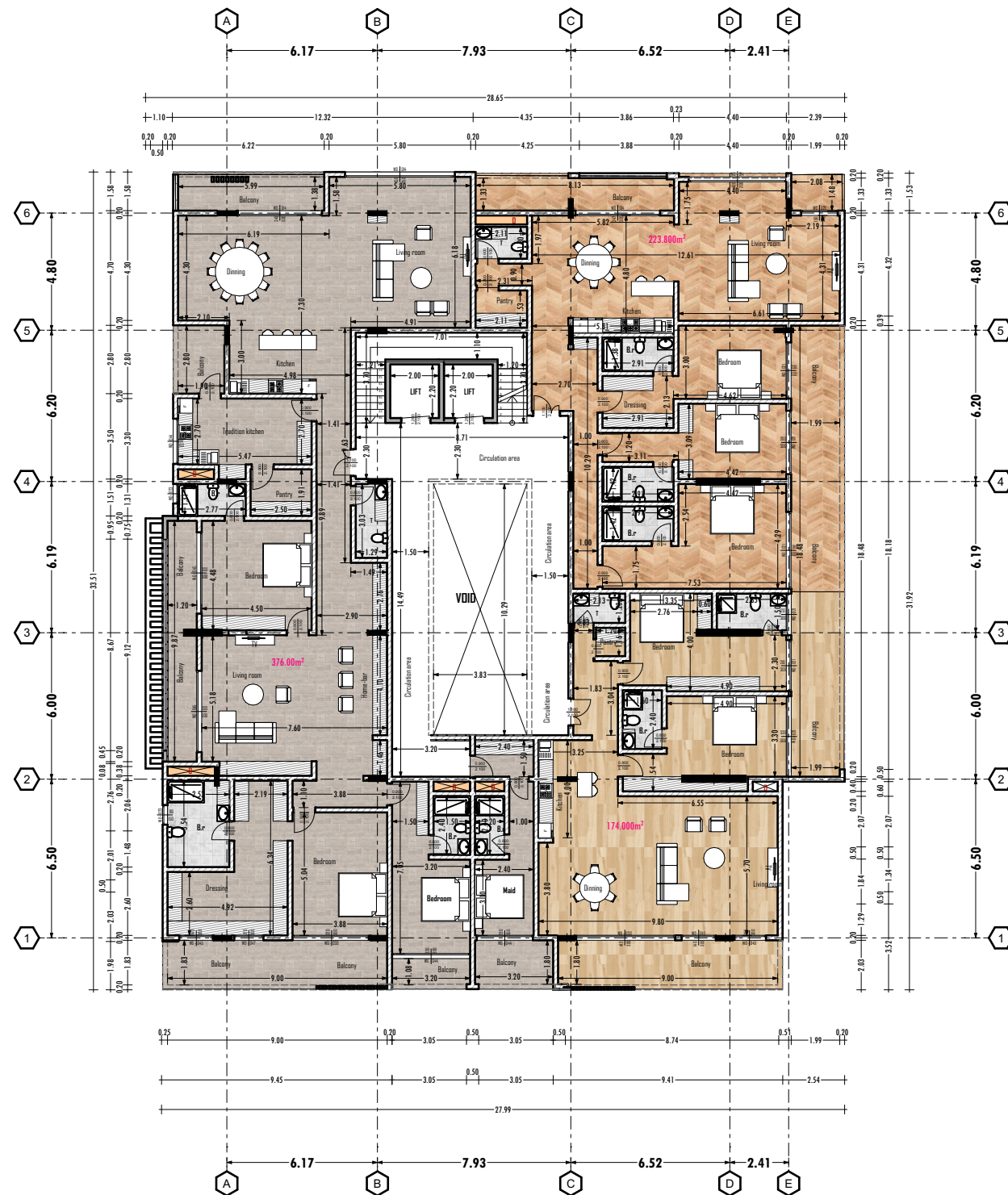
FOURTH FLOOR PLAN LAYOUT
