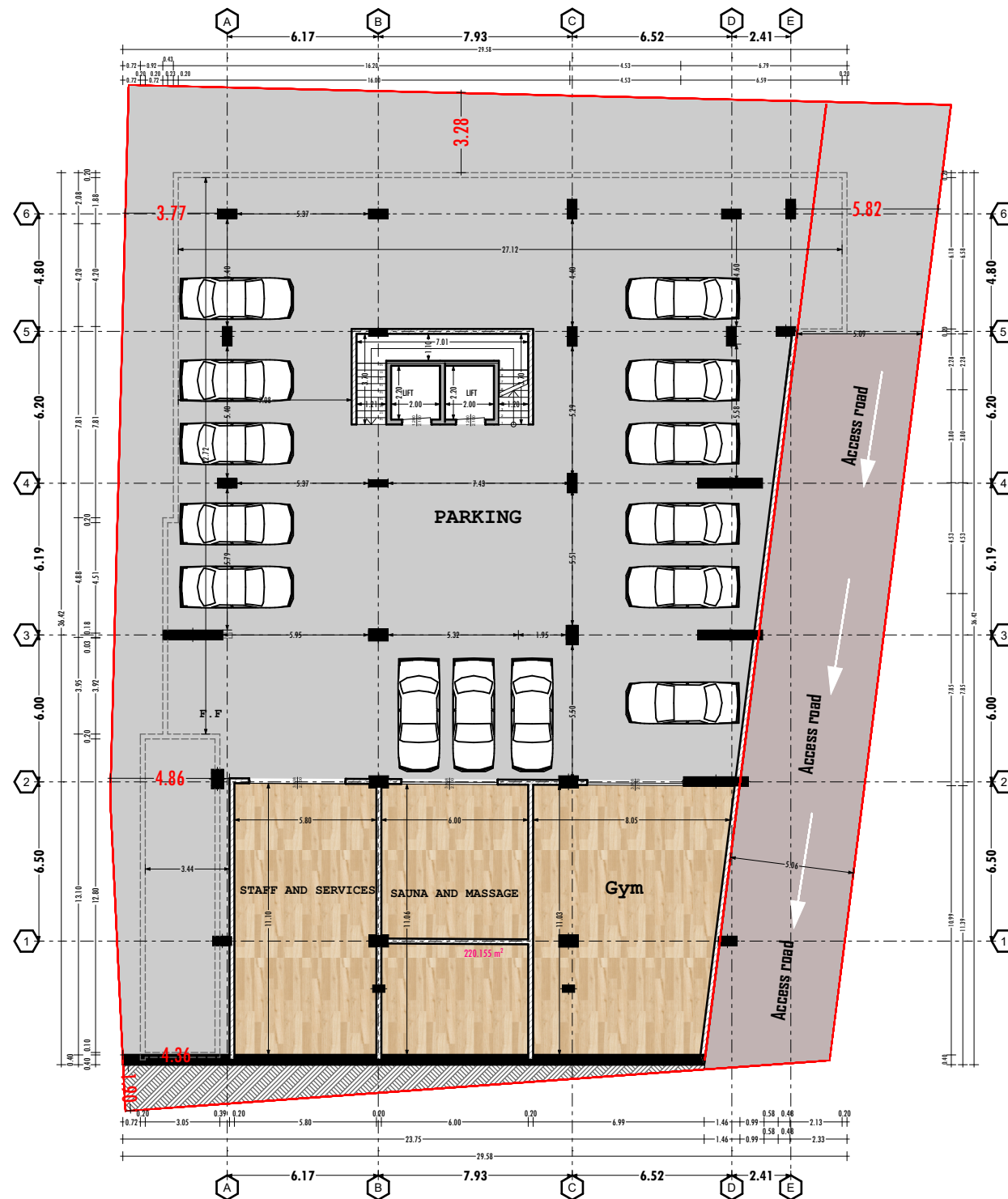
BASEMENT FLOOR PLAN LAYOUT
