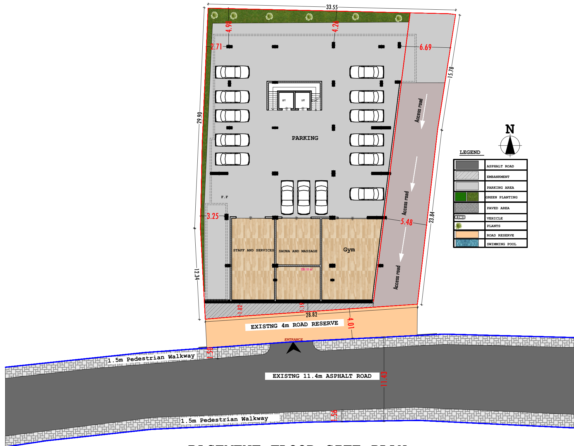
BASEMENT FLOOR SITE PLAN
